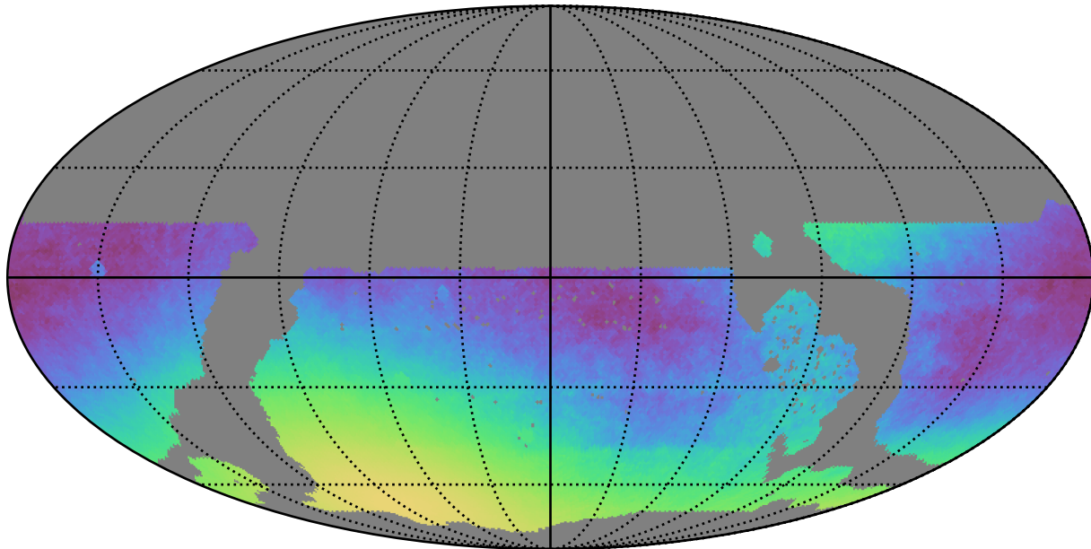
ddf_loaded_fl4_v3.4_10yrs WFD: Normalized Parallax Uncert @ 22.4
