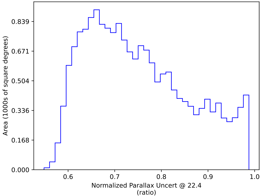
ddf_loaded_fl4_v3.4_10yrs WFD: Normalized Parallax Uncert @ 22.4
