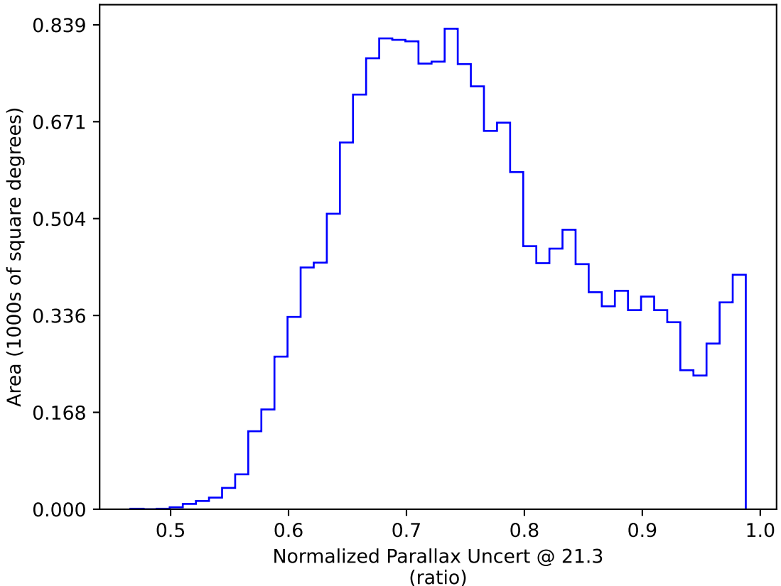
ddf_loaded_fl4_v3.4_10yrs WFD y band only: Normalized Parallax Uncert @ 21.3
