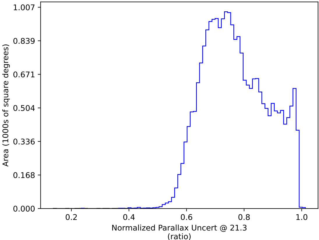
ddf_loaded_fl4_v3.4_10yrs All sky y band only: Normalized Parallax Uncert @ 21.3
