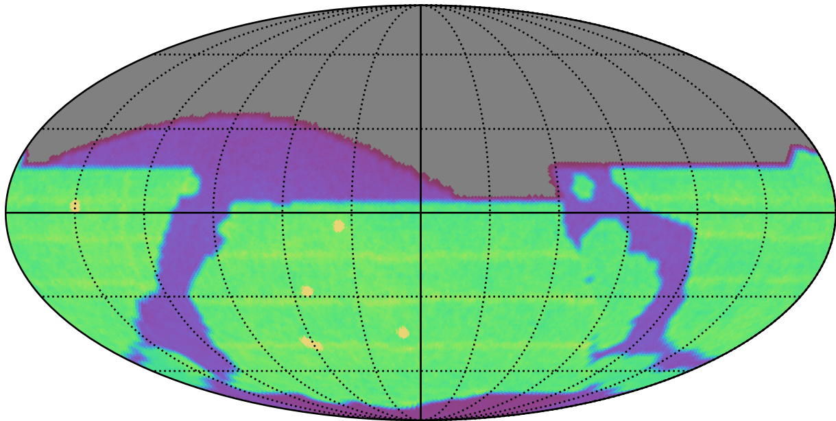
ddf_loaded_fl4_v3.4_10yrs All sky all bands: N Unique Nights
