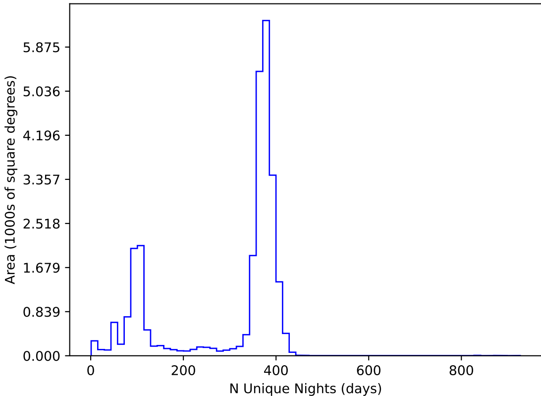
ddf_loaded_fl4_v3.4_10yrs All sky all bands: N Unique Nights
