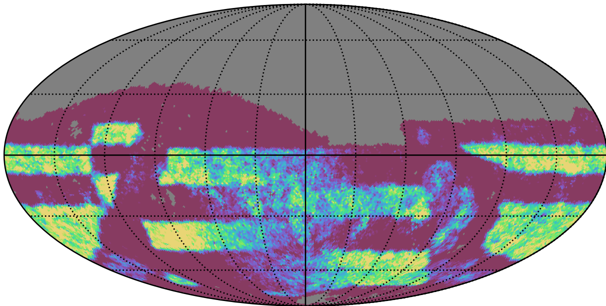
ddf_loaded_fl4_v3.4_10yrs Yr 3-4 z band: NVisits
