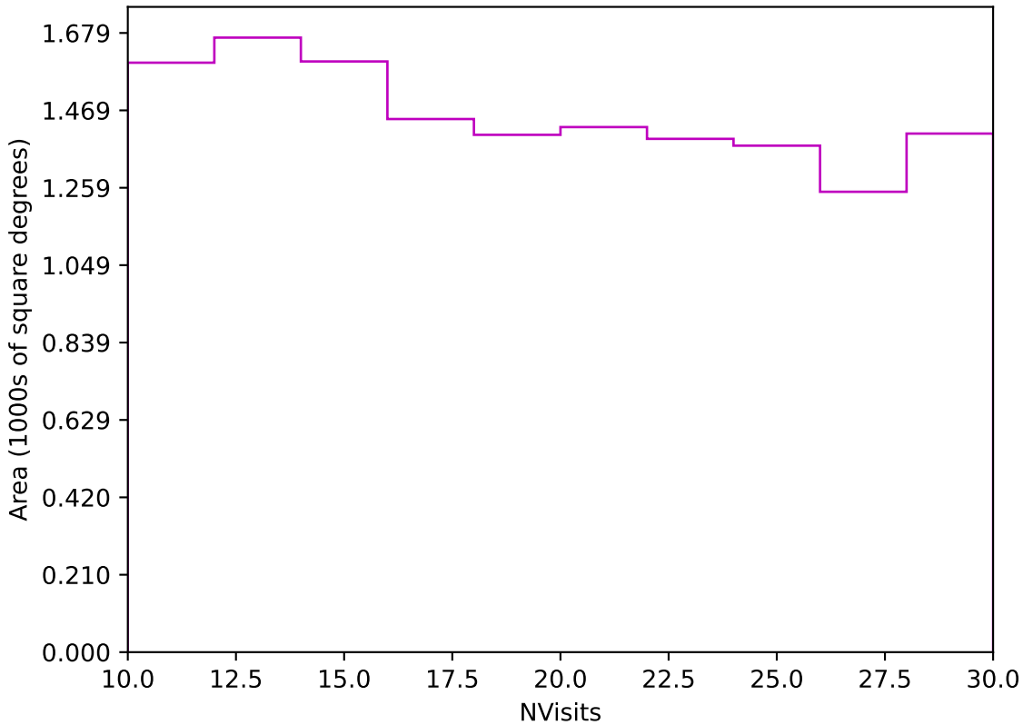
ddf_loaded_fl4_v3.4_10yrs Yr 3-4 z band: NVisits
