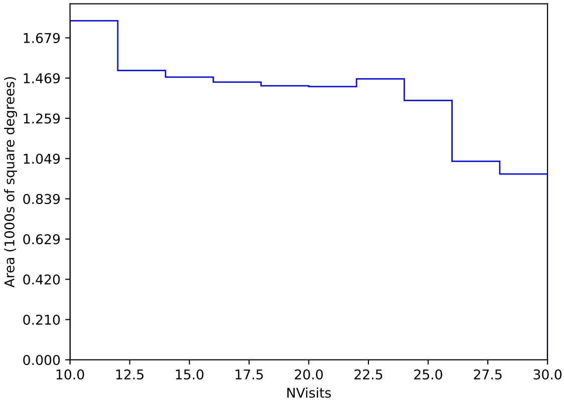
ddf_loaded_fl4_v3.4_10yrs Yr 3-4 y band: NVisits
