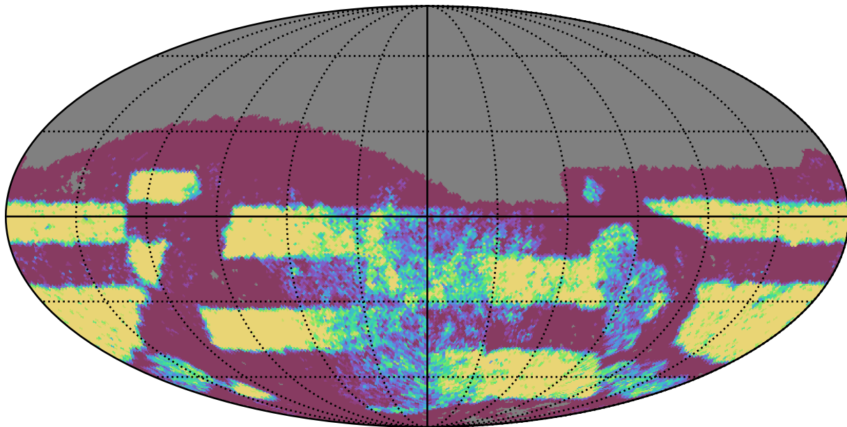
ddf_loaded_fl4_v3.4_10yrs Yr 3-4 i band: NVisits
