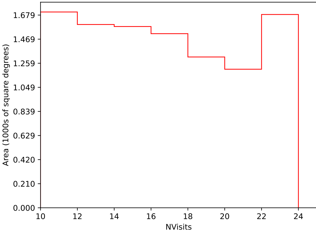
ddf_loaded_fl4_v3.4_10yrs Yr 3-4 i band: NVisits
