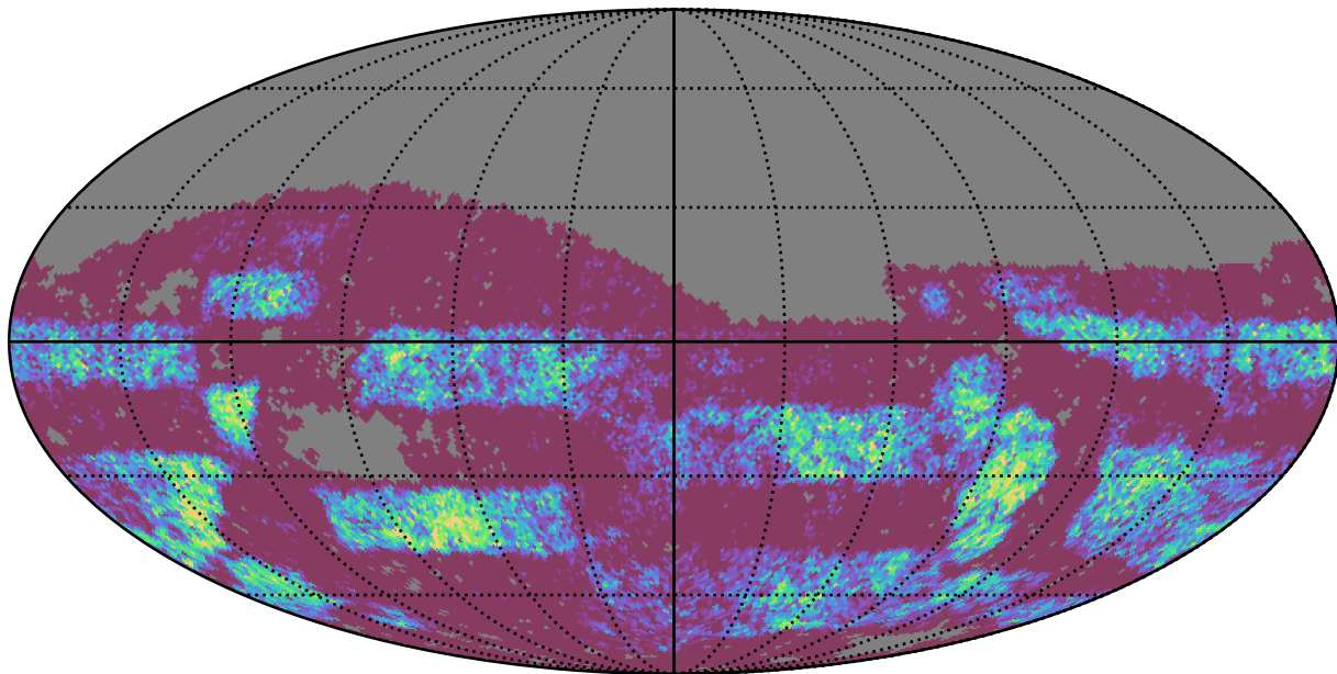
ddf_loaded_fl4_v3.4_10yrs Yr 3-4 g band: NVisits
