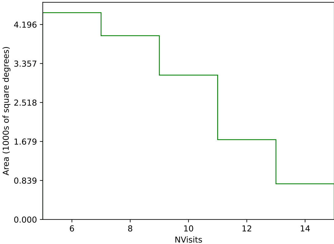
ddf_loaded_fl4_v3.4_10yrs Yr 3-4 g band: NVisits
