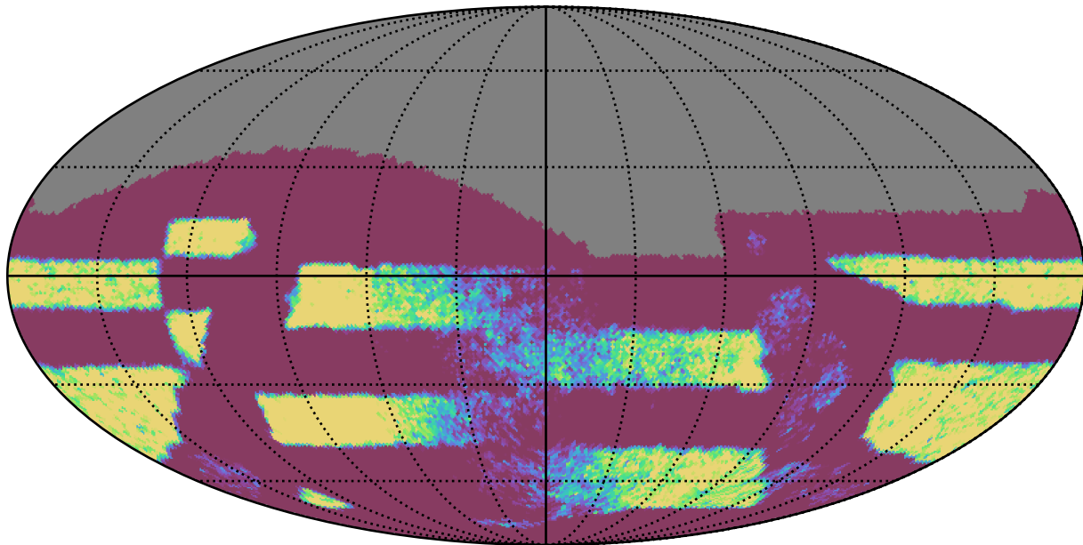
ddf_loaded_fl4_v3.4_10yrs Yr 3-4 all bands: NVisits
