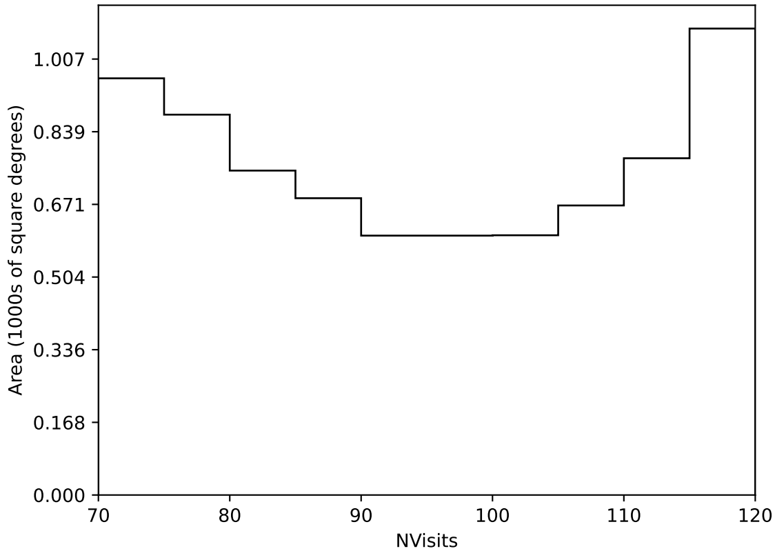
ddf_loaded_fl4_v3.4_10yrs Yr 3-4 all bands: NVisits
