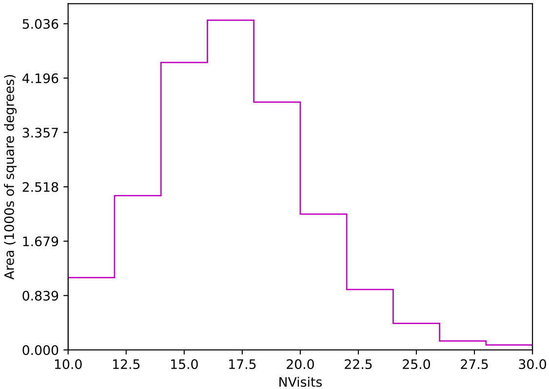
ddf_loaded_fl4_v3.4_10yrs Yr 1 z band: NVisits
