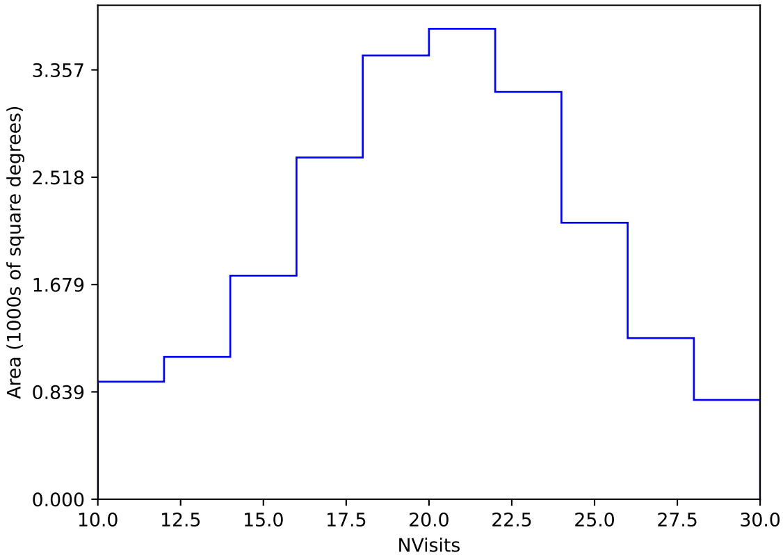
ddf_loaded_fl4_v3.4_10yrs Yr 1 y band: NVisits
