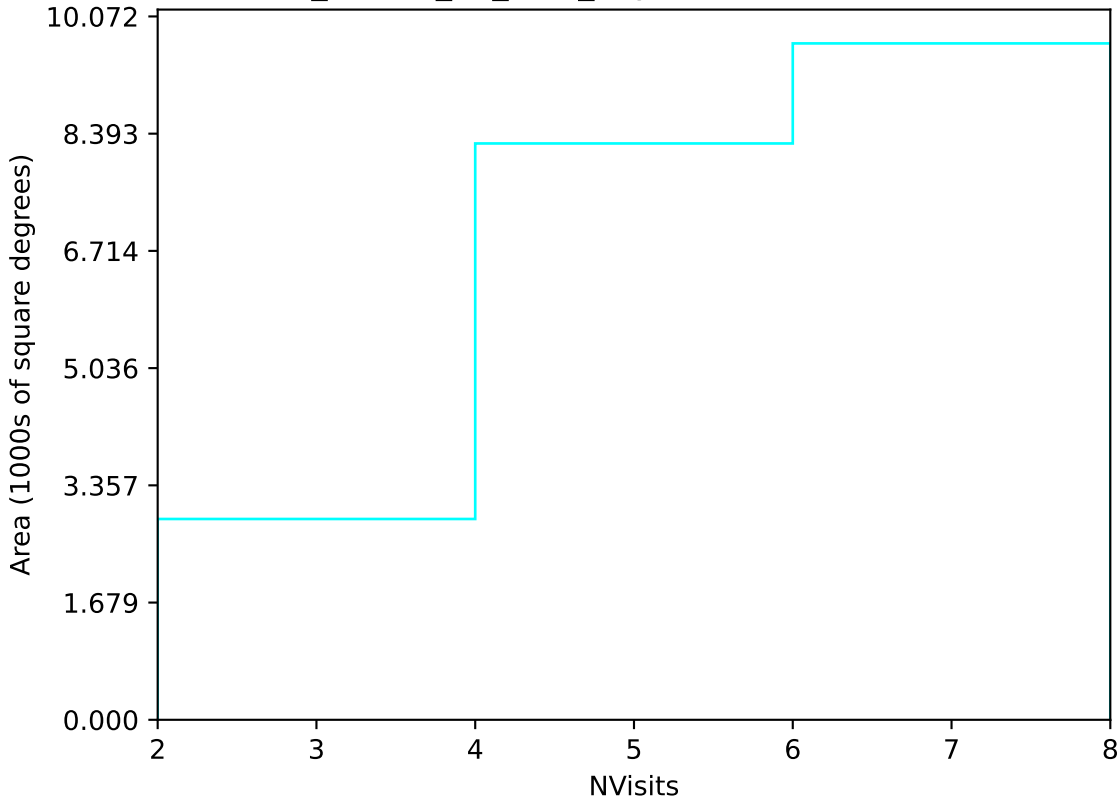
ddf_loaded_fl4_v3.4_10yrs Yr 1 u band: NVisits
