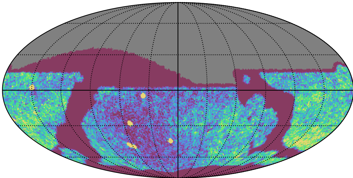
ddf_loaded_fl4_v3.4_10yrs Yr 1 all bands: NVisits
