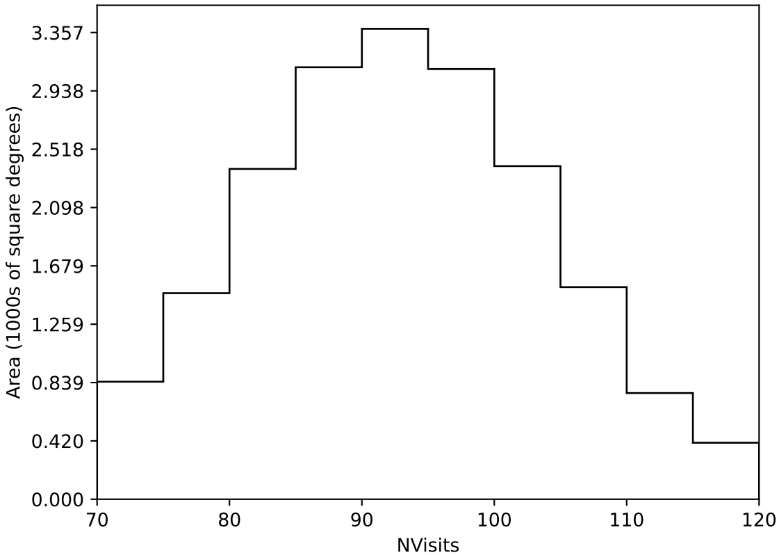
ddf_loaded_fl4_v3.4_10yrs Yr 1 all bands: NVisits
