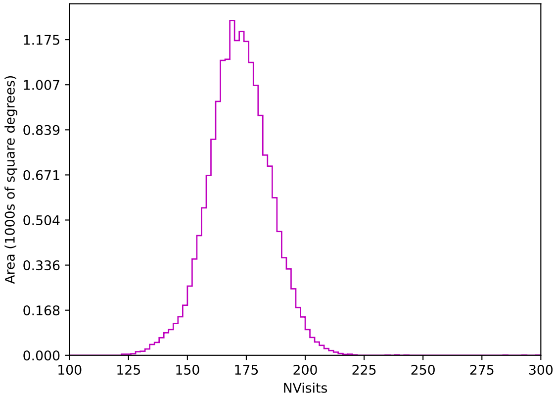
ddf_loaded_fl4_v3.4_10yrs WFD z band: NVisits
