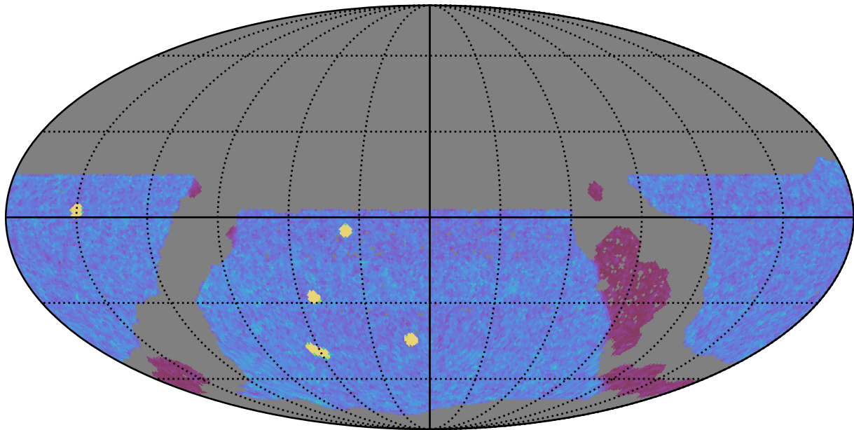
ddf_loaded_fl4_v3.4_10yrs WFD y band: NVisits
