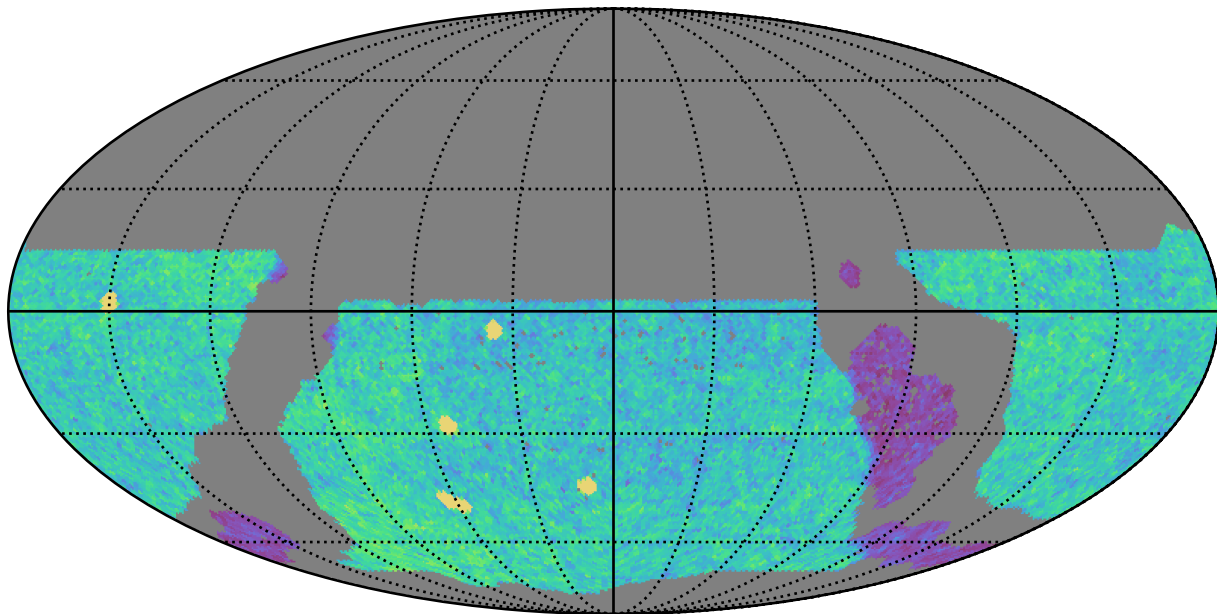
ddf_loaded_fl4_v3.4_10yrs WFD u band: NVisits
