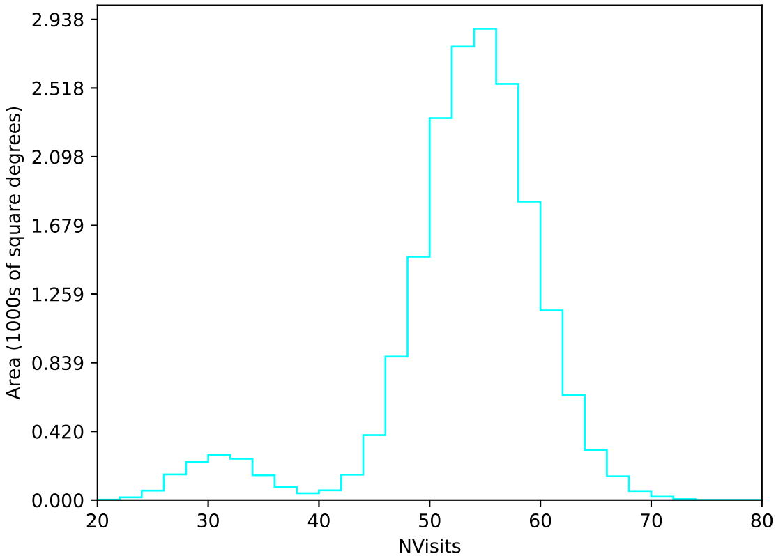
ddf_loaded_fl4_v3.4_10yrs WFD u band: NVisits
