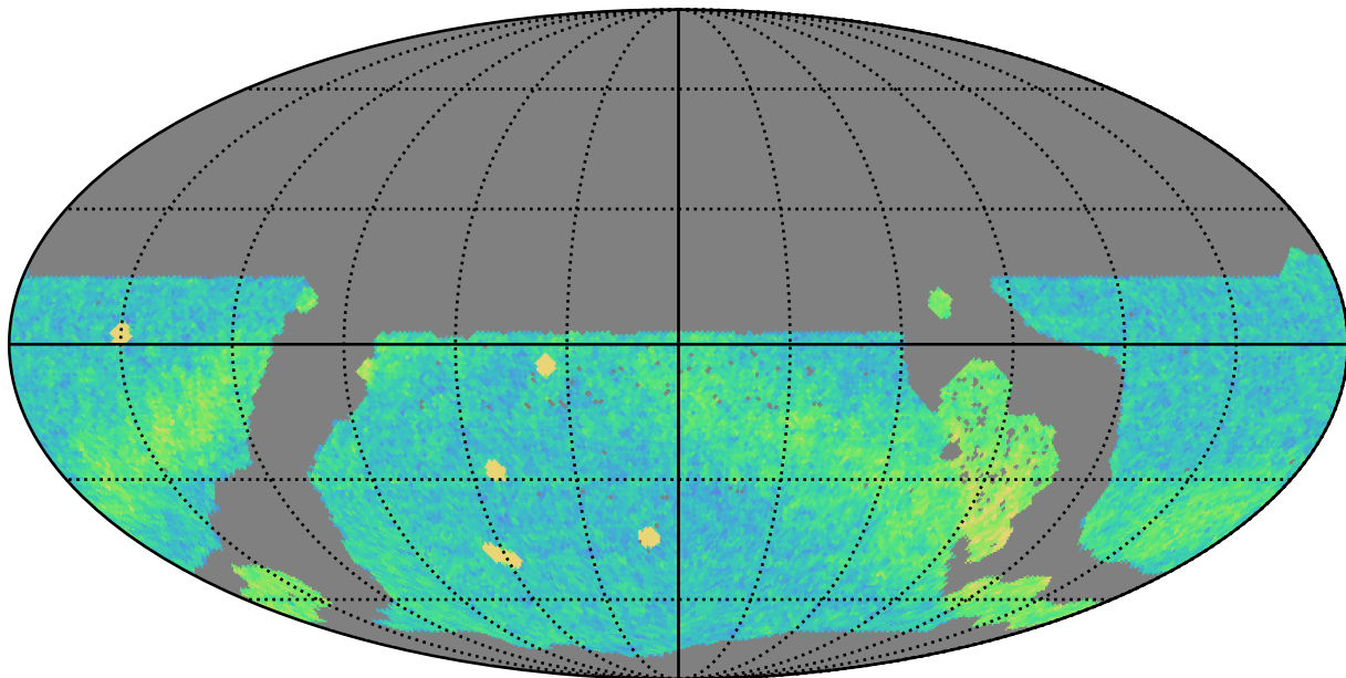
ddf_loaded_fl4_v3.4_10yrs WFD r band: NVisits
