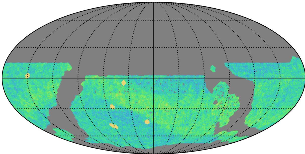
ddf_loaded_fl4_v3.4_10yrs WFD i band: NVisits
