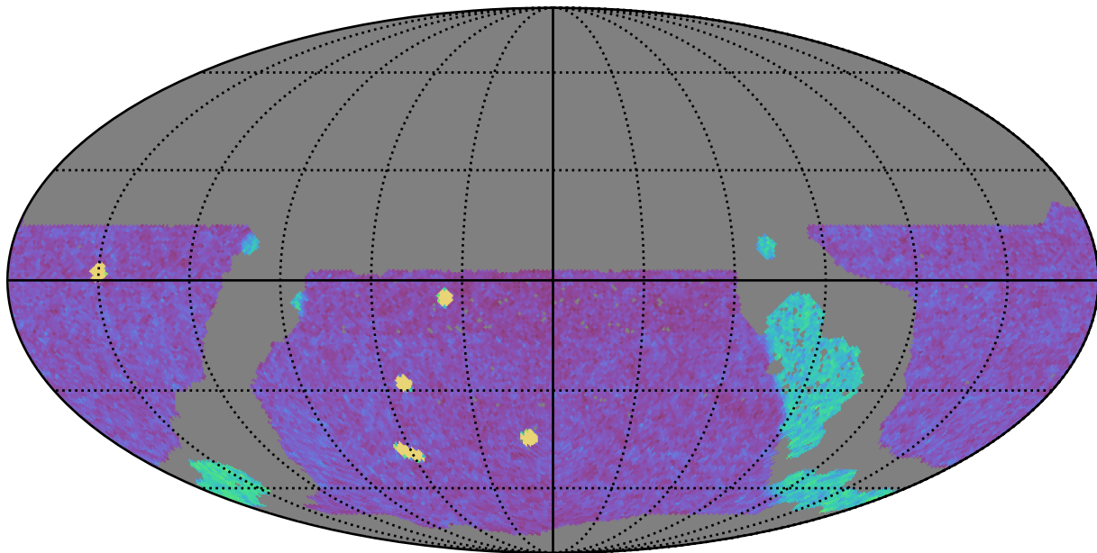
ddf_loaded_fl4_v3.4_10yrs WFD g band: NVisits
