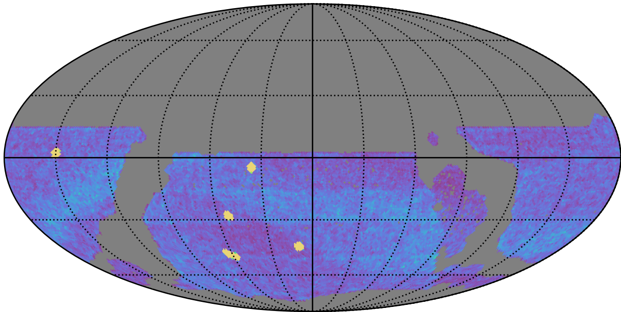
ddf_loaded_fl4_v3.4_10yrs WFD all bands: NVisits
