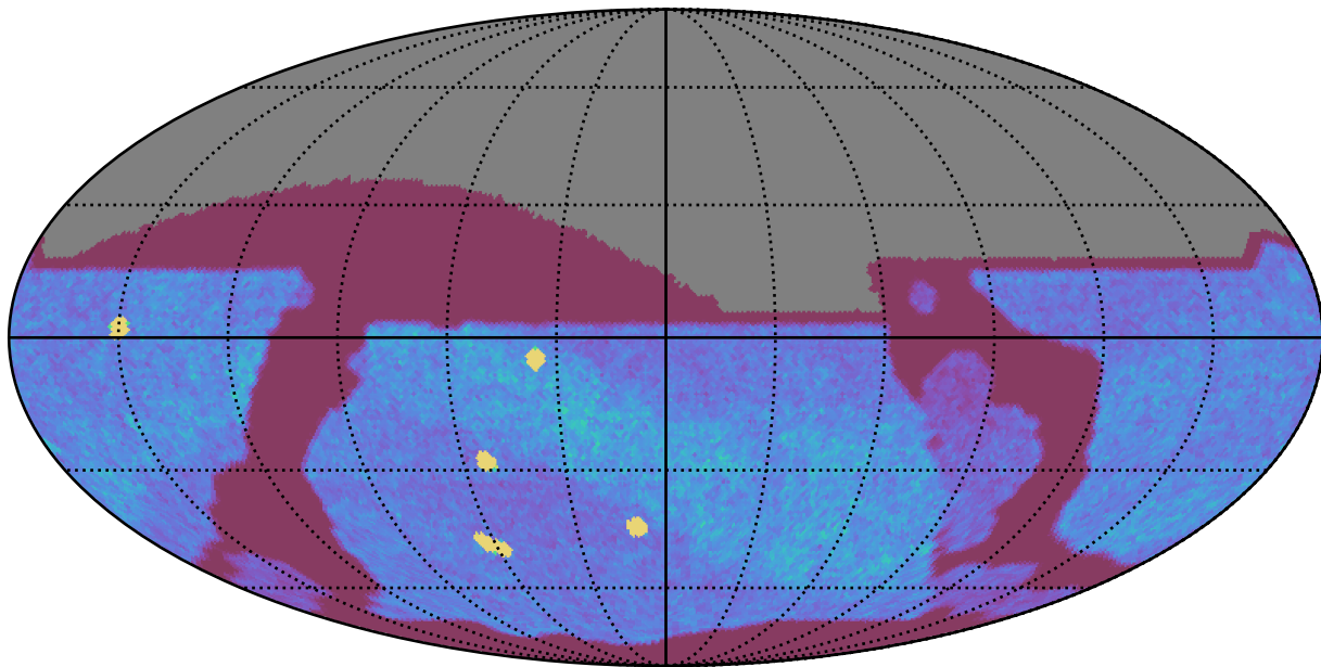
ddf_loaded_fl4_v3.4_10yrs All sky z band: NVisits
