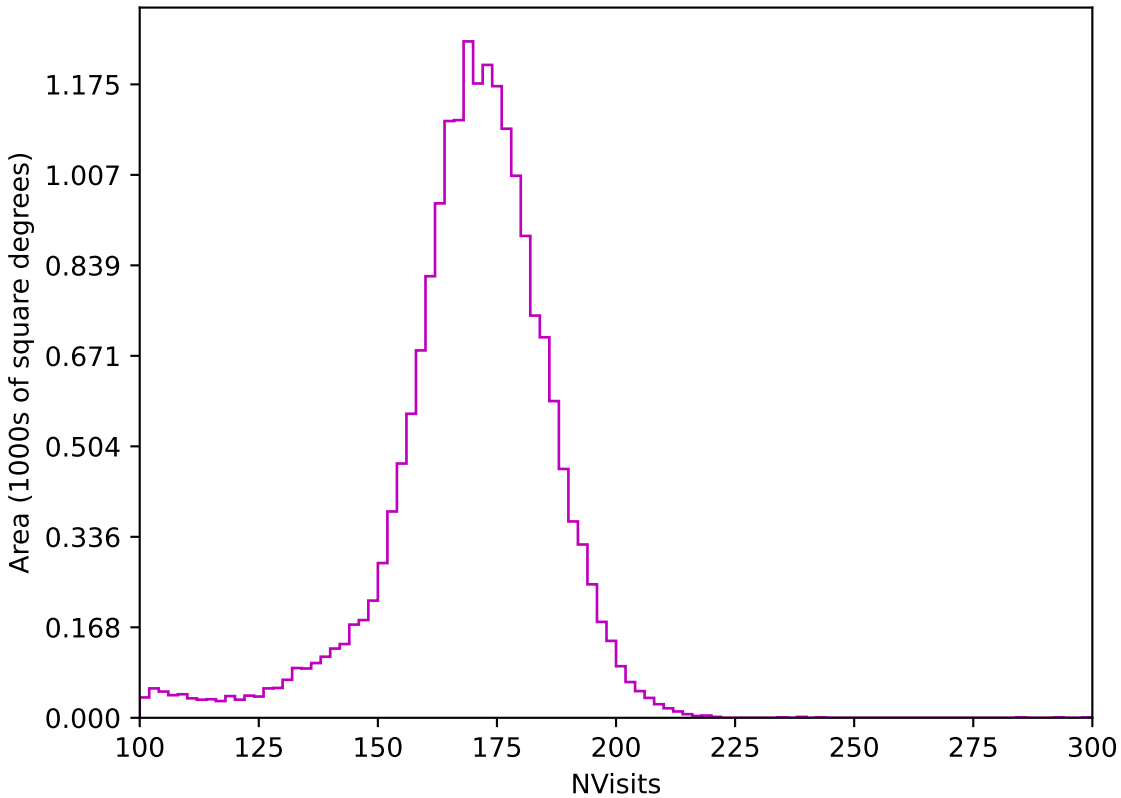
ddf_loaded_fl4_v3.4_10yrs All sky z band: NVisits
