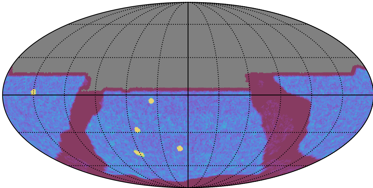
ddf_loaded_fl4_v3.4_10yrs All sky y band: NVisits
