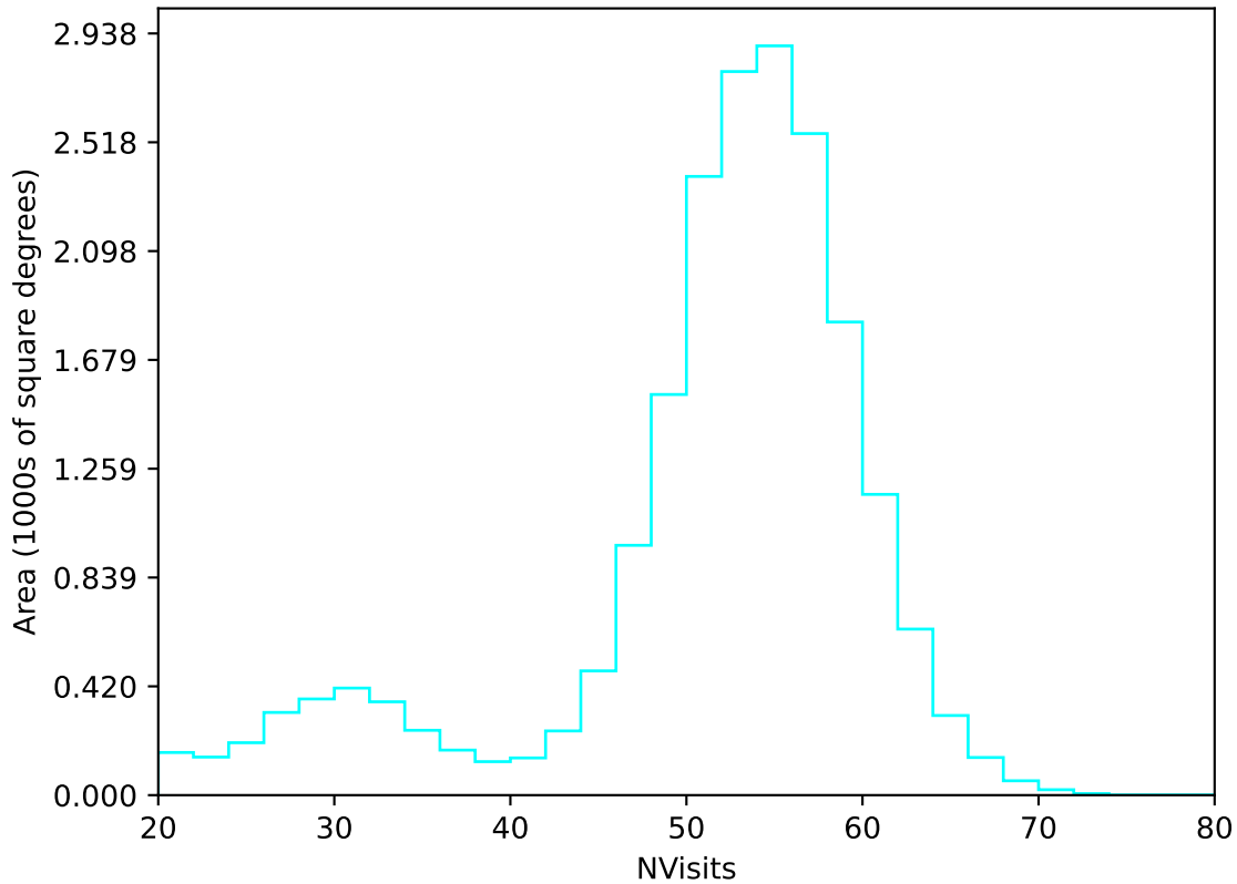
ddf_loaded_fl4_v3.4_10yrs All sky u band: NVisits
