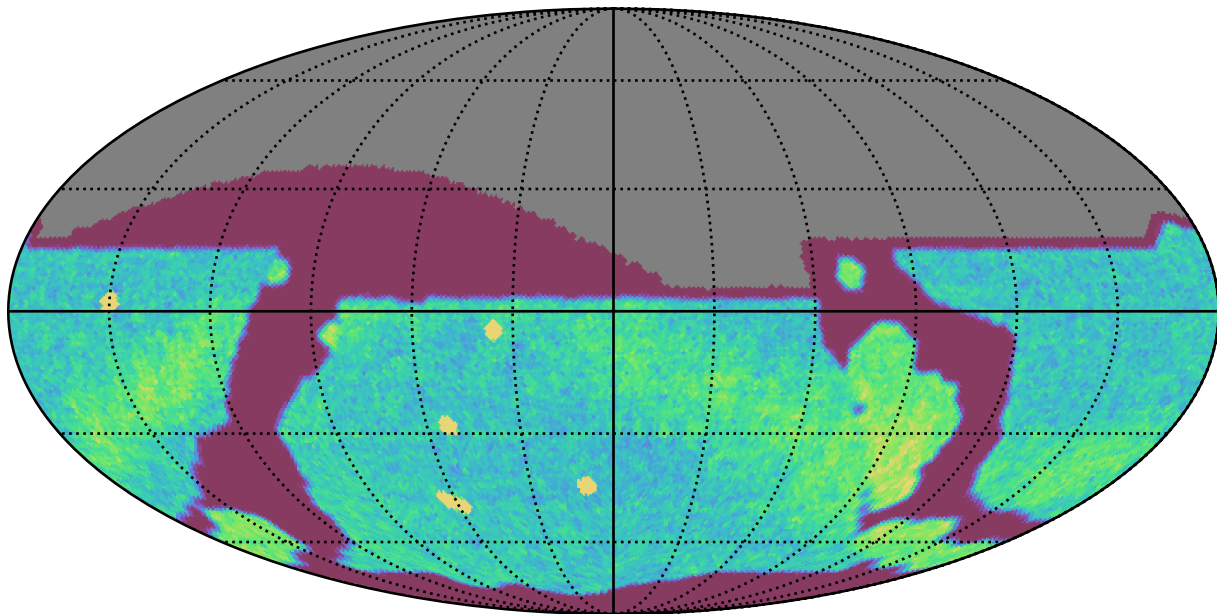
ddf_loaded_fl4_v3.4_10yrs All sky r band: NVisits
