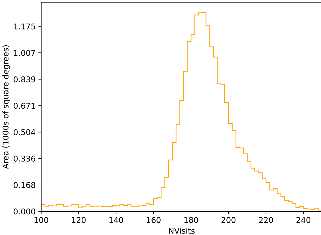
ddf_loaded_fl4_v3.4_10yrs All sky r band: NVisits
