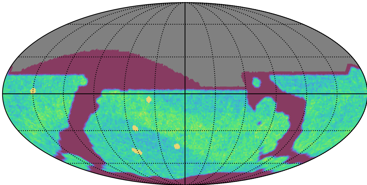
ddf_loaded_fl4_v3.4_10yrs All sky i band: NVisits
