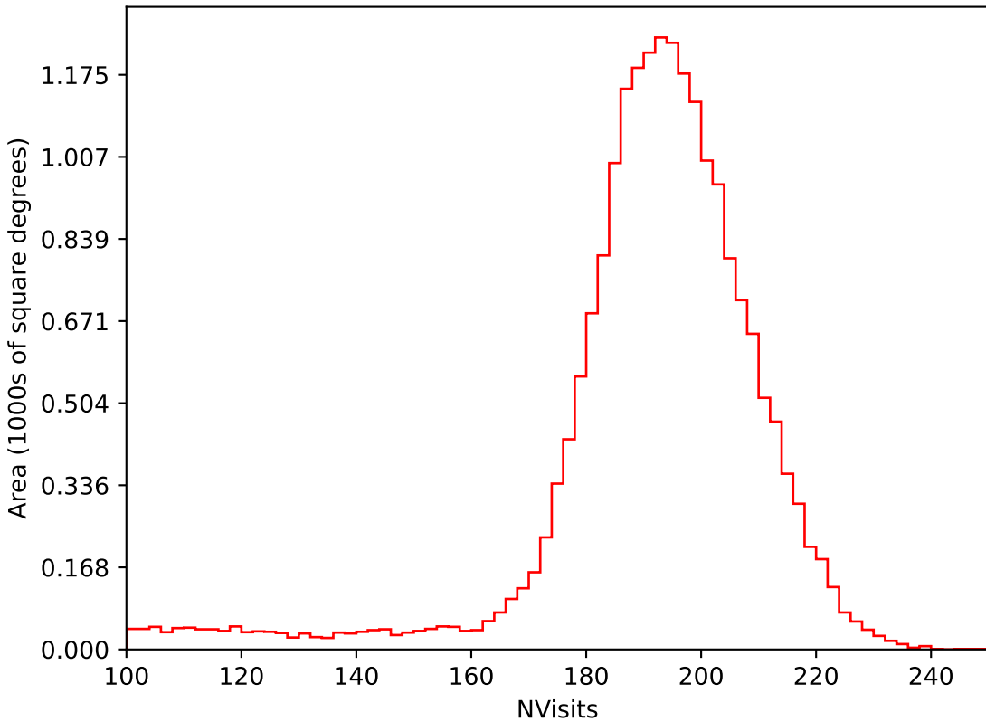
ddf_loaded_fl4_v3.4_10yrs All sky i band: NVisits
