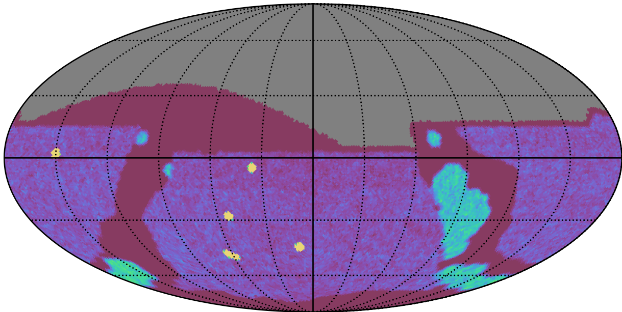
ddf_loaded_fl4_v3.4_10yrs All sky g band: NVisits
