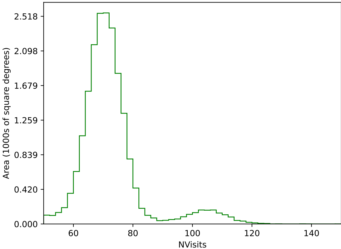
ddf_loaded_fl4_v3.4_10yrs All sky g band: NVisits
