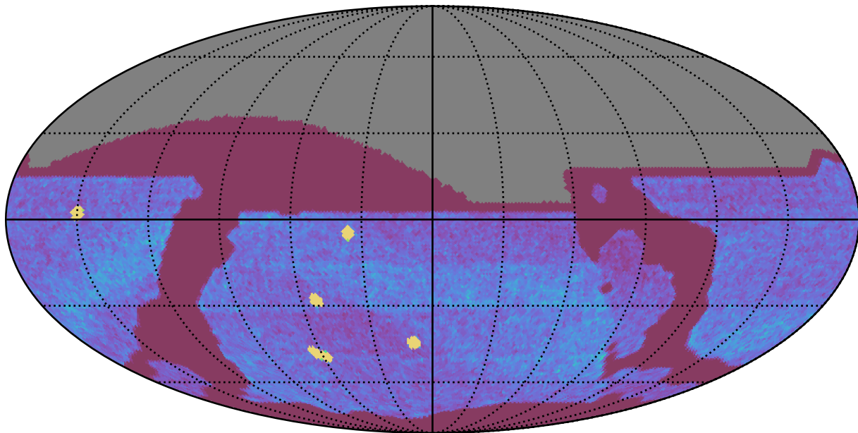
ddf_loaded_fl4_v3.4_10yrs All sky all bands: NVisits
