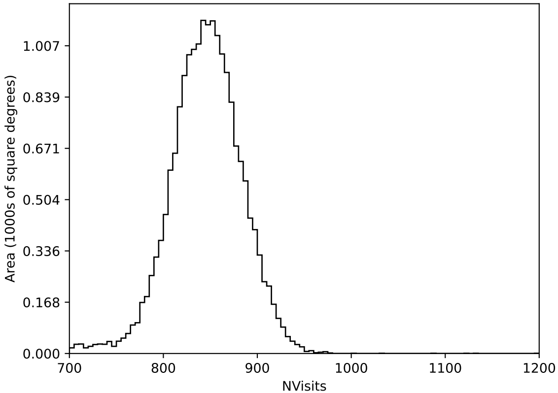
ddf_loaded_fl4_v3.4_10yrs All sky all bands: NVisits
