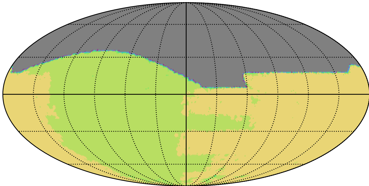
ddf_loaded_fl4_v3.4_10yrs All sky all bands: NSeasons
