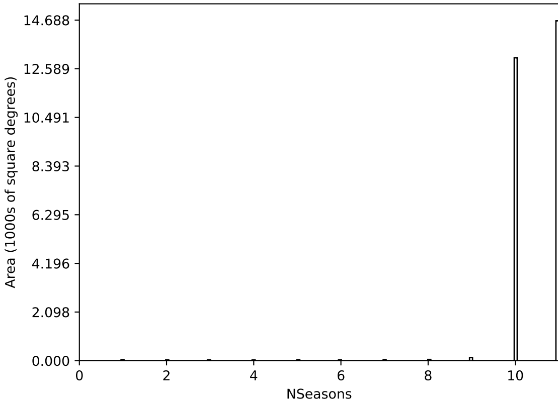
ddf_loaded_fl4_v3.4_10yrs All sky all bands: NSeasons
