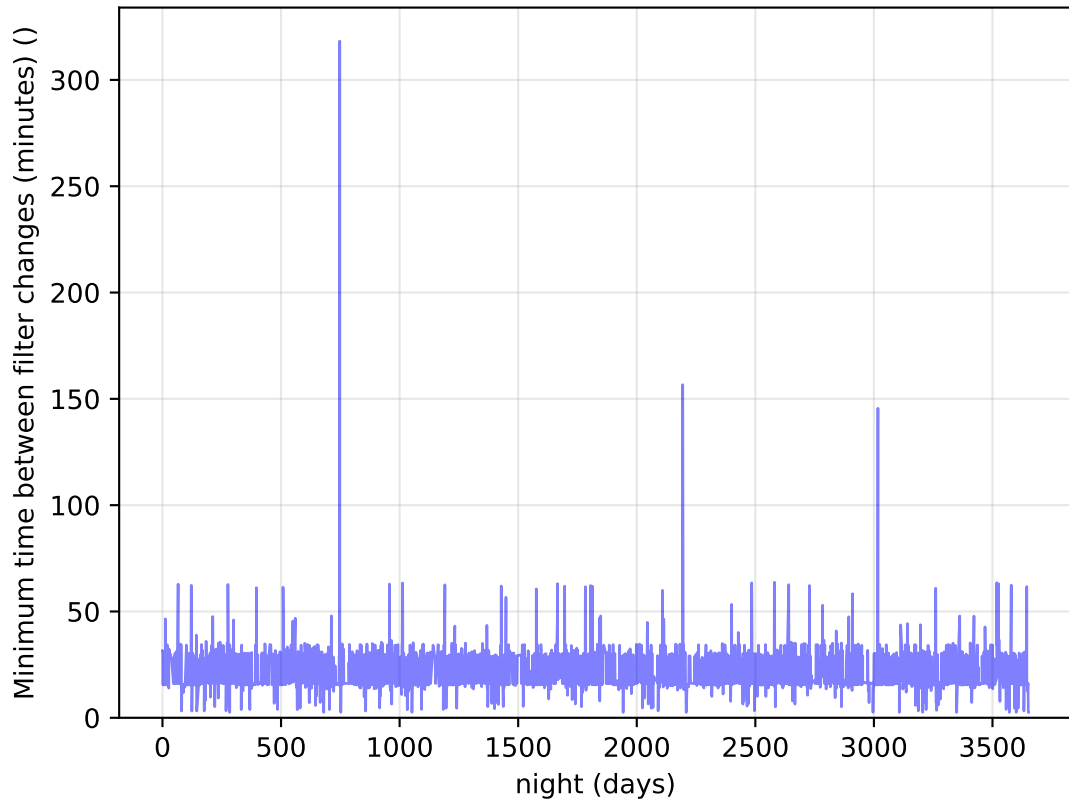
ddf_loaded_fl4_v3.4_10yrs Per Night: Minimum time between filter changes (minutes)
