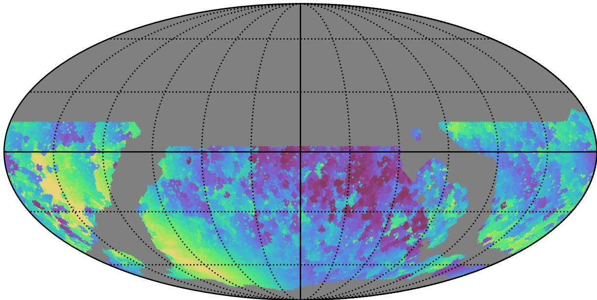
ddf_loaded_fl4_v3.4_10yrs WFD y band: Min solarElong
