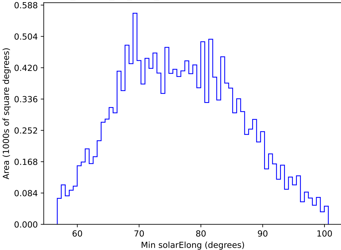
ddf_loaded_fl4_v3.4_10yrs WFD u band: Min solarElong
