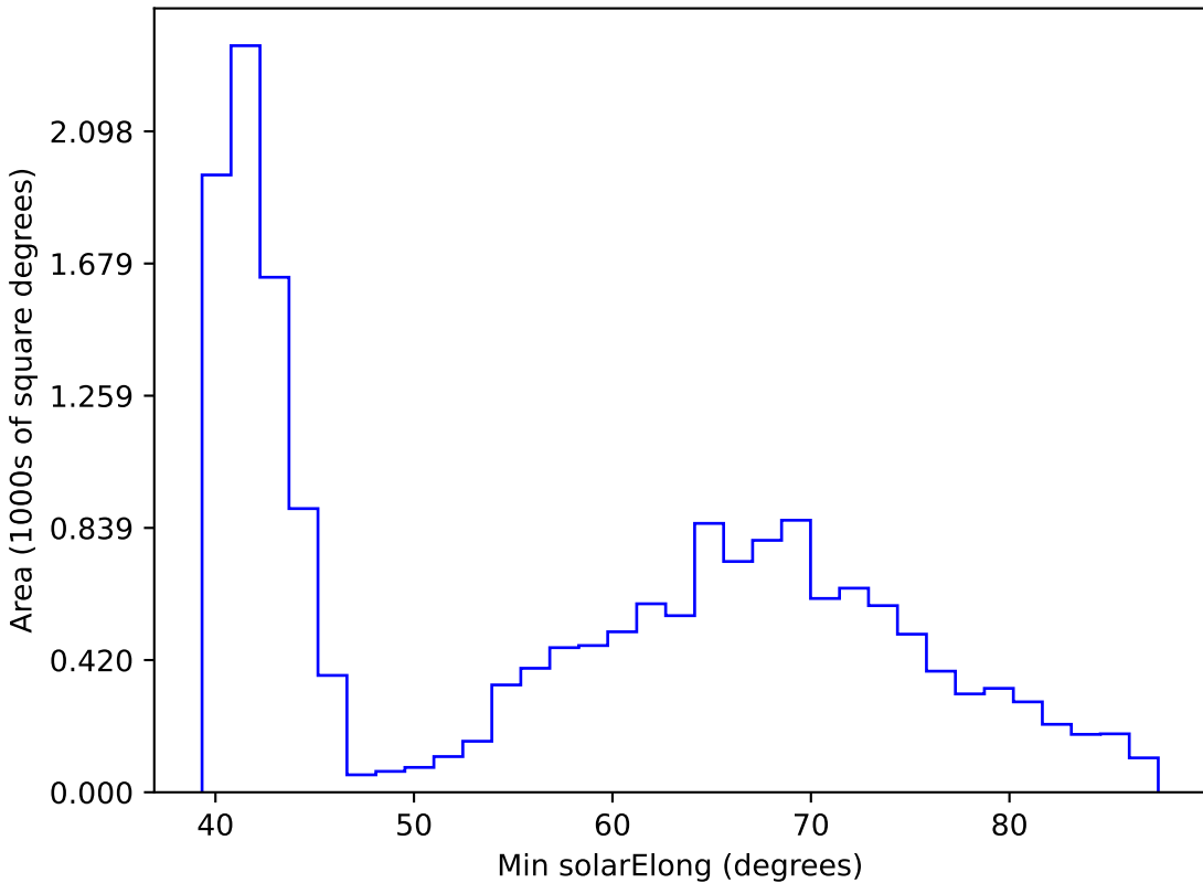
ddf_loaded_fl4_v3.4_10yrs WFD r band: Min solarElong
