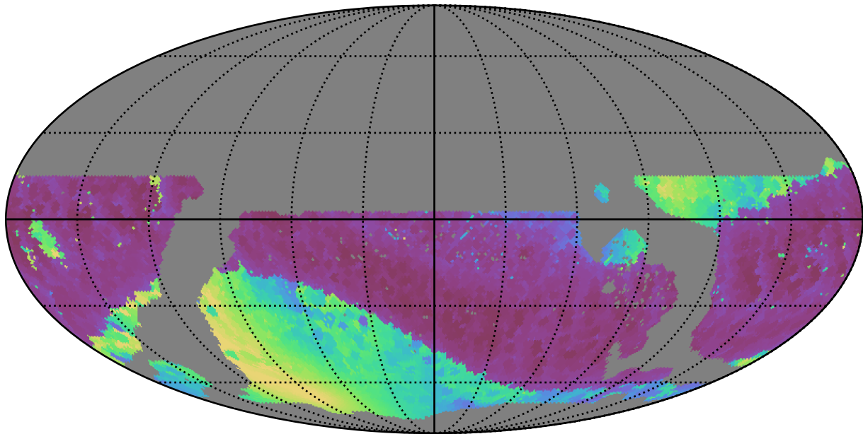
ddf_loaded_fl4_v3.4_10yrs WFD i band: Min solarElong
