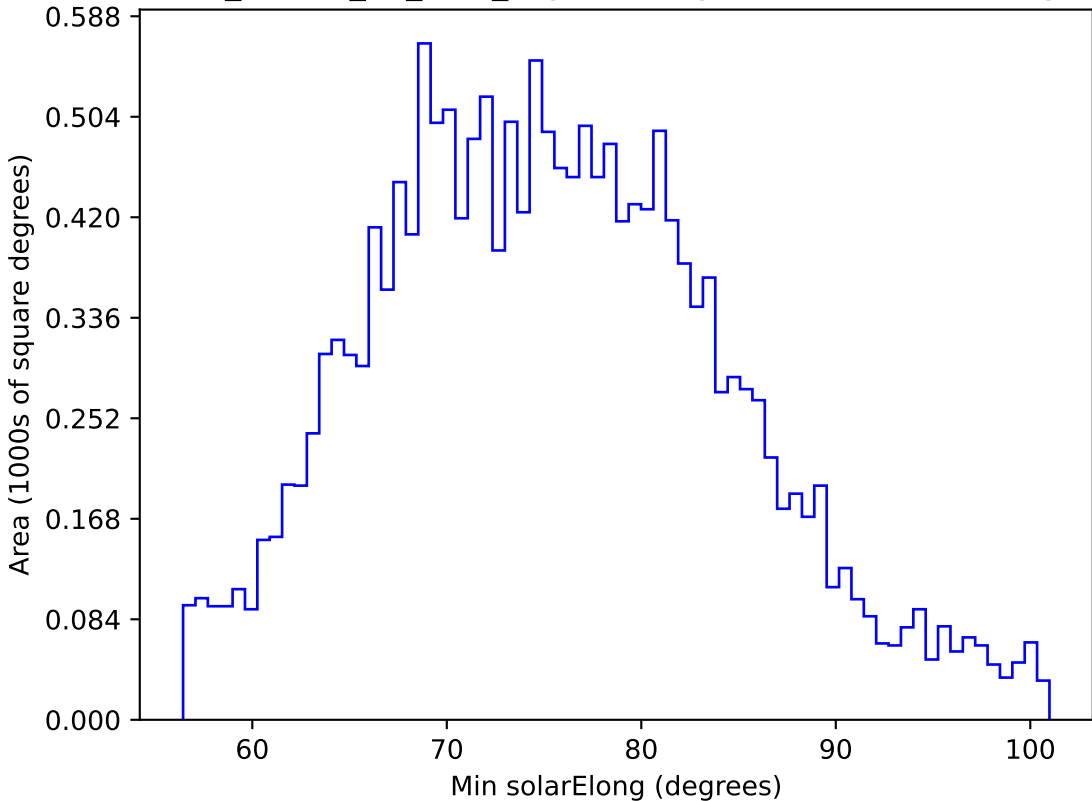
ddf_loaded_fl4_v3.4_10yrs WFD g band: Min solarElong
