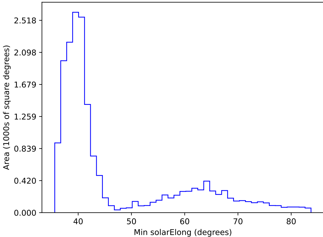
ddf_loaded_fl4_v3.4_10yrs WFD all bands: Min solarElong
