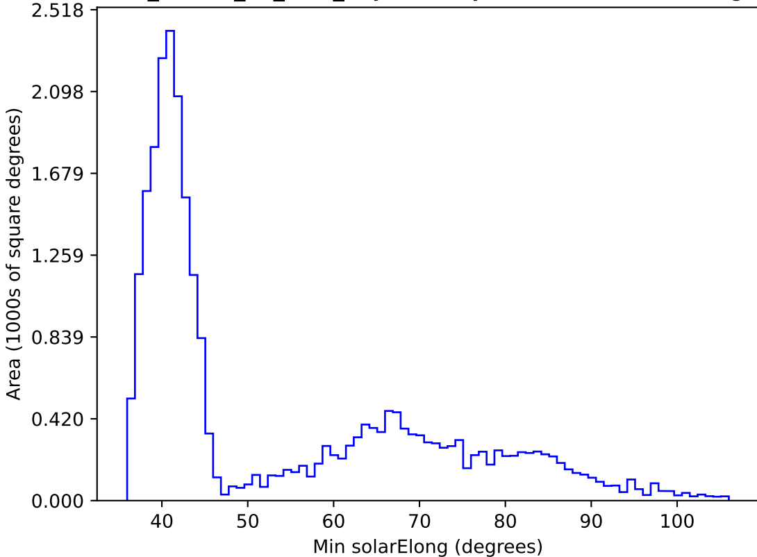
ddf_loaded_fl4_v3.4_10yrs All sky z band: Min solarElong
